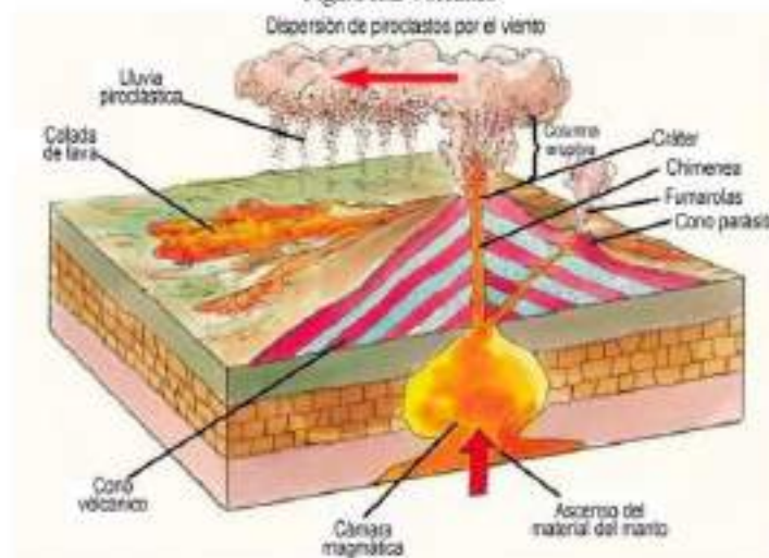
Figura II.2 Volcanes
